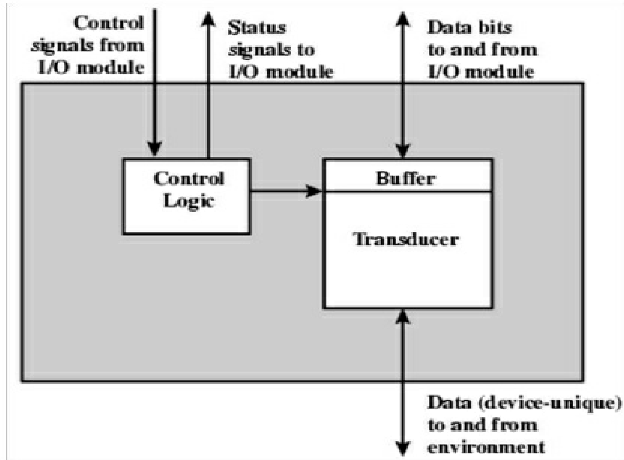
Figure: External I/O Module Diagram
